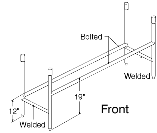
940 Series Cross Bracing
