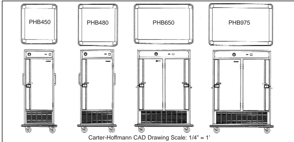
Carter-Hoffmann CAD Drawing Scale: 1/4" = 1'
